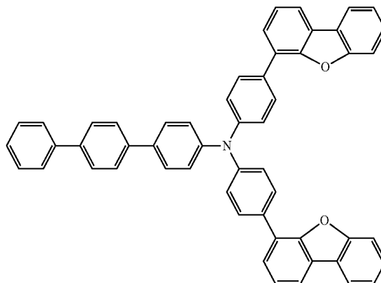
Chemical Formula 2-2
