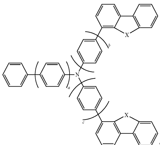
Chemical Formula 2
