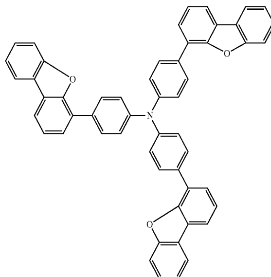
Chemical Formula 1-1
