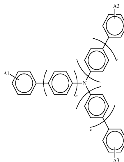
Chemical Formula 1
