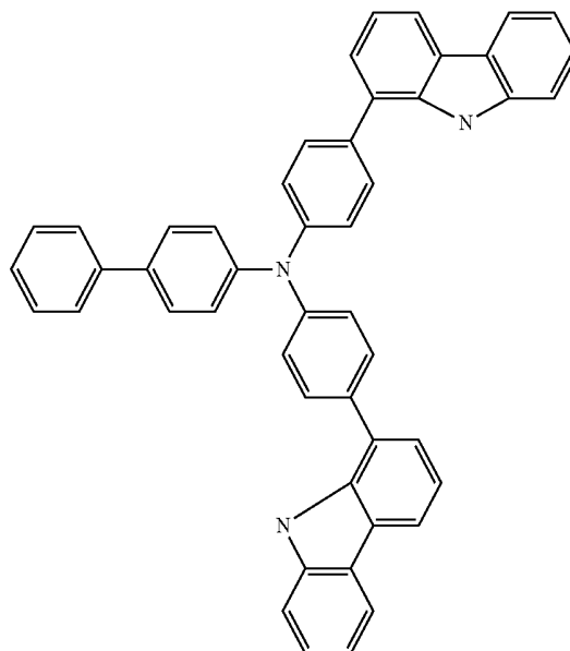
Chemical Formula 2-3
