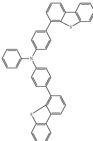
Chemical Formula 1-5
