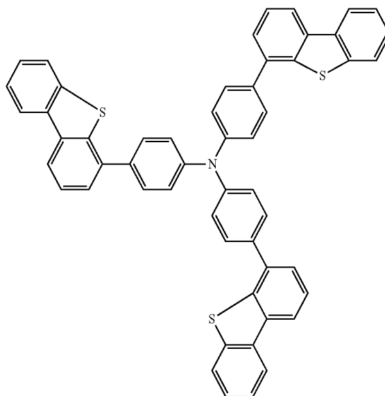
Chemical Formula 1-4
