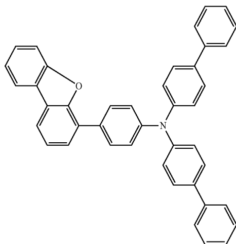
Chemical Formula 1-3
