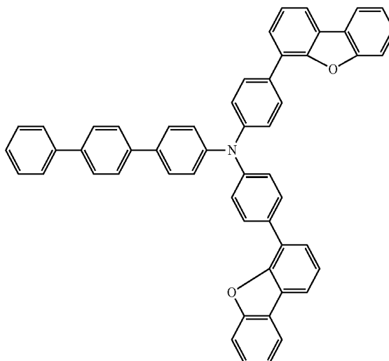
Chemical Formula 2-3
