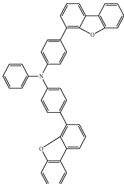
Chemical Formula 1-2
